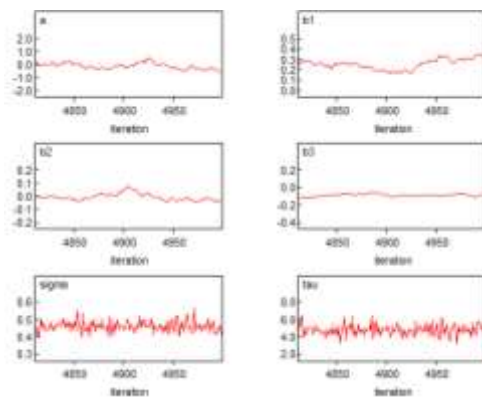
Gambar 2. Trace plot
