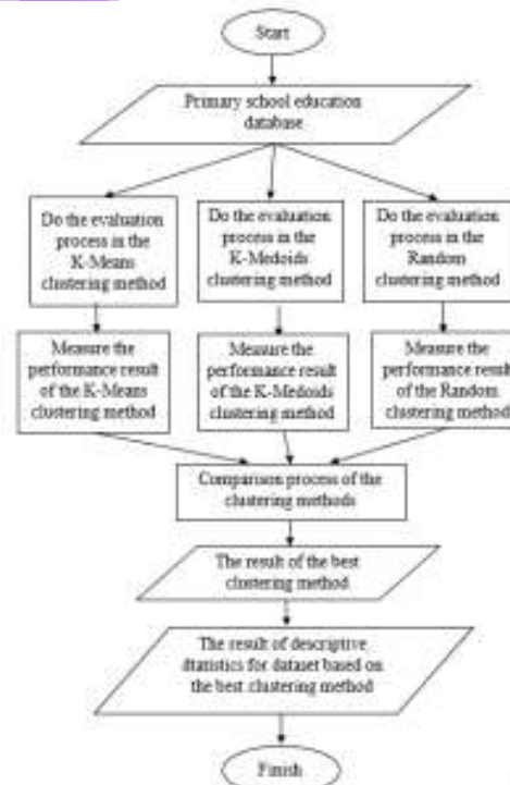
Figure 2. Flowchart of clustering comparison.
