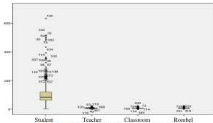
Figure 3. Boxplot results of research variables.
