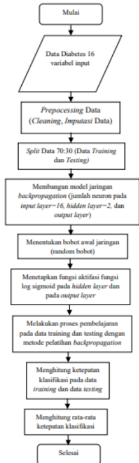
Gambar 1 Flow Chart DLNN
