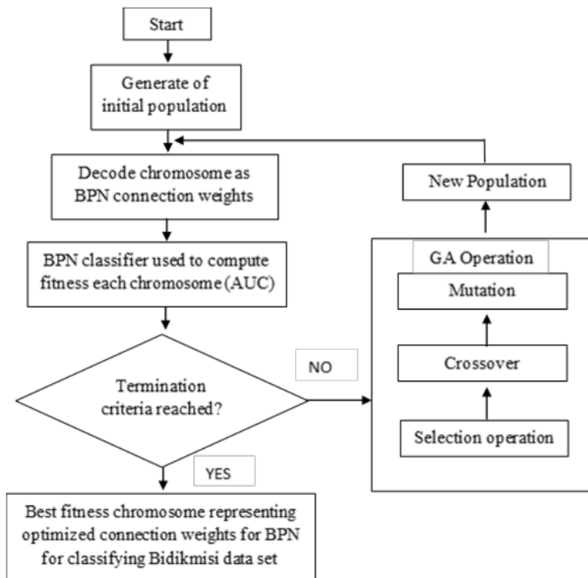
Figure 1. Working of hybrid BPNGA
