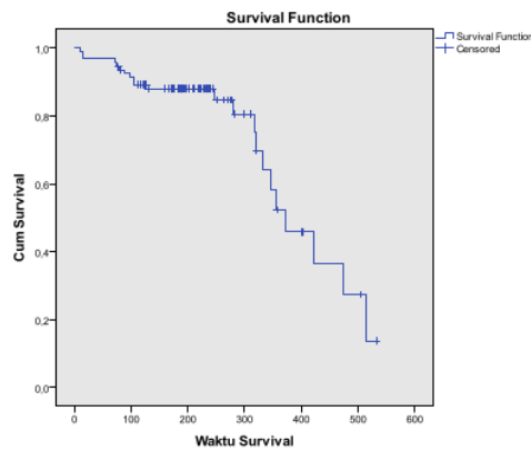
Figure 1: Survival probability curve for breast cancer patients
