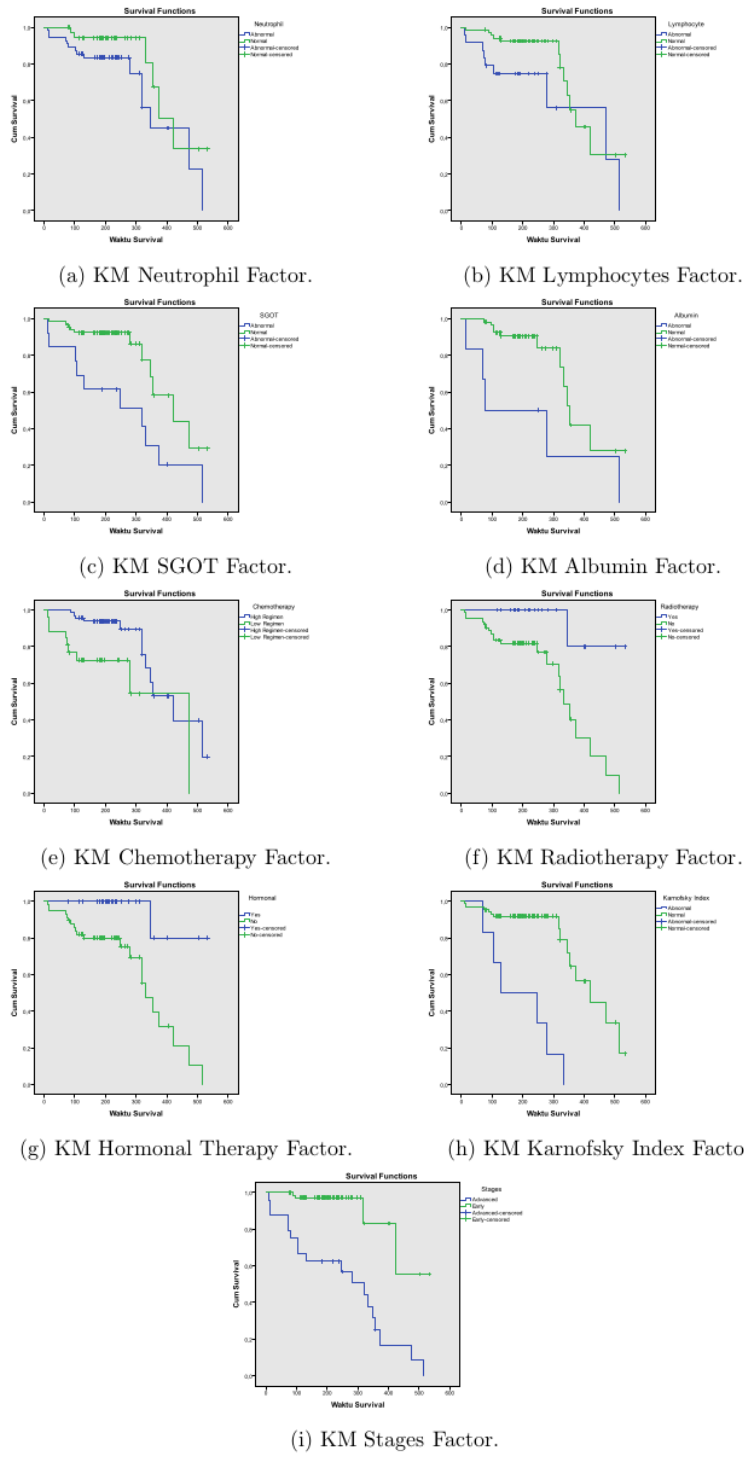
Figure 2: Survival probability curve based on variables.
